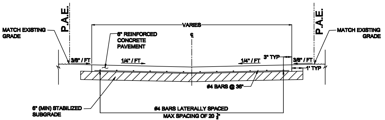
SECTION B-B CONCRETE PAVEMENT
