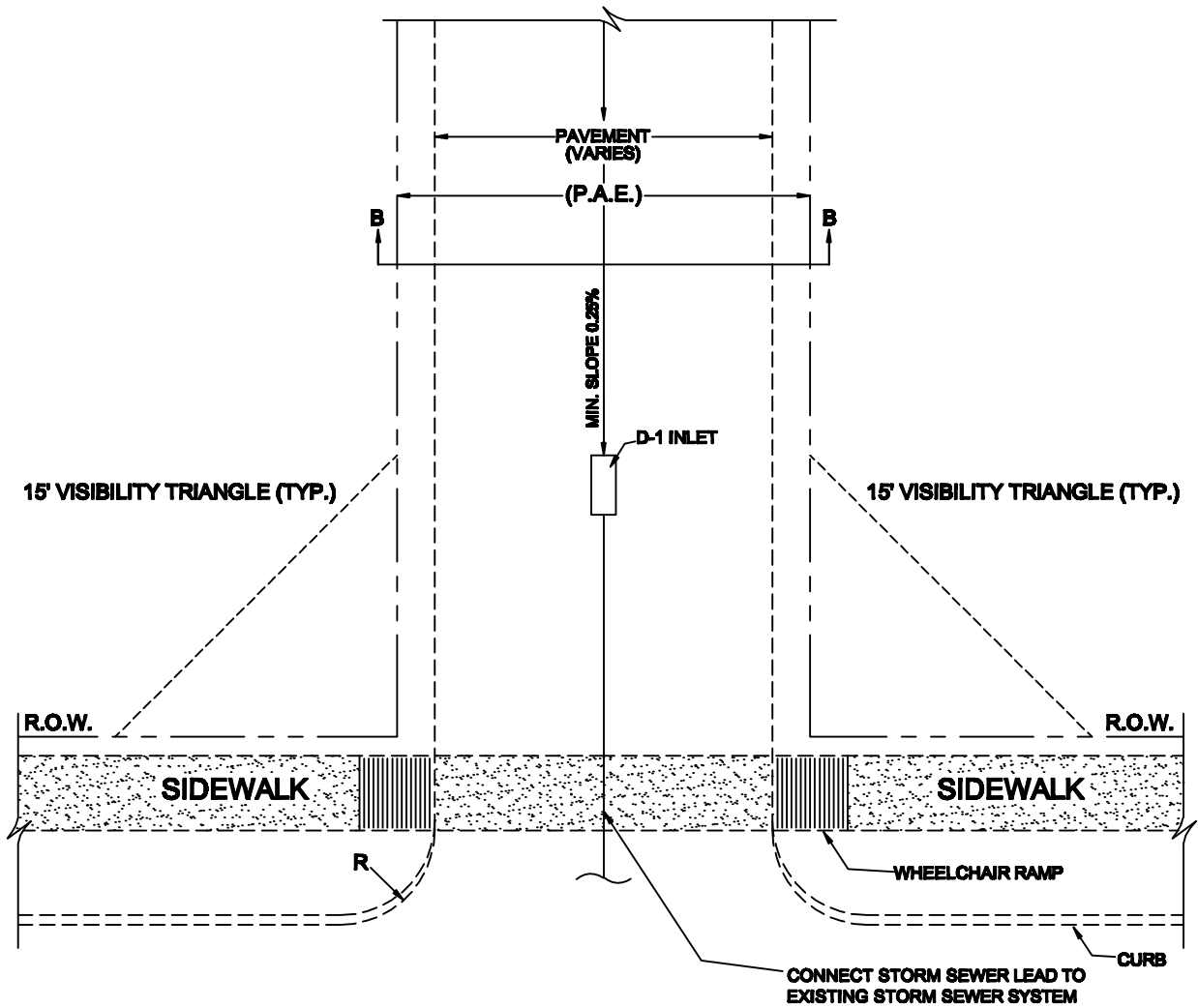
PLAN VIEW
